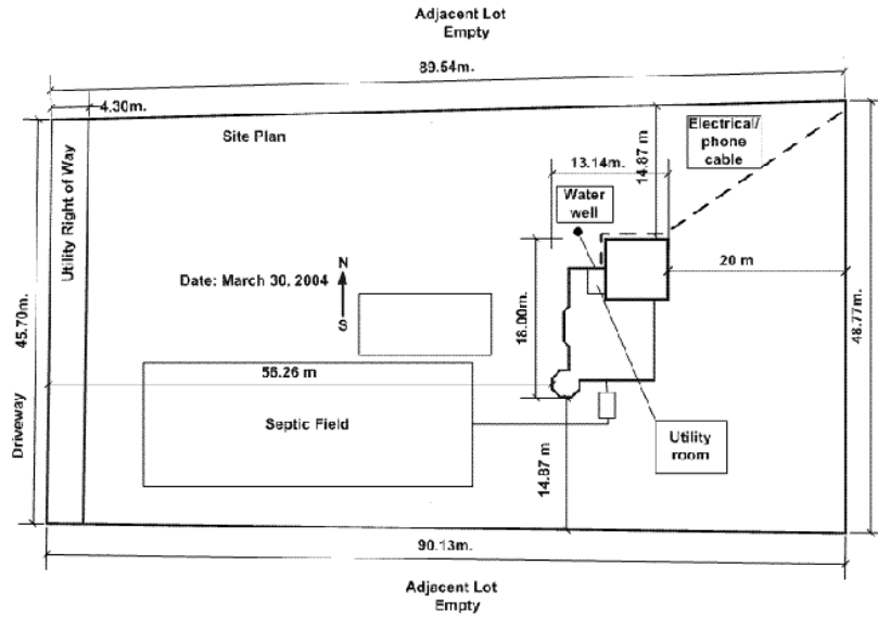
Example Septic Field sketch
