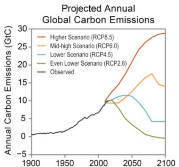
Figure 17: Carbon emissions through the 21st century (2000-2100) for four greenhouse gas emission scenarios, or Representative Concentration Pathways, developed by the Intergovernmental Panel on Climate Change.
