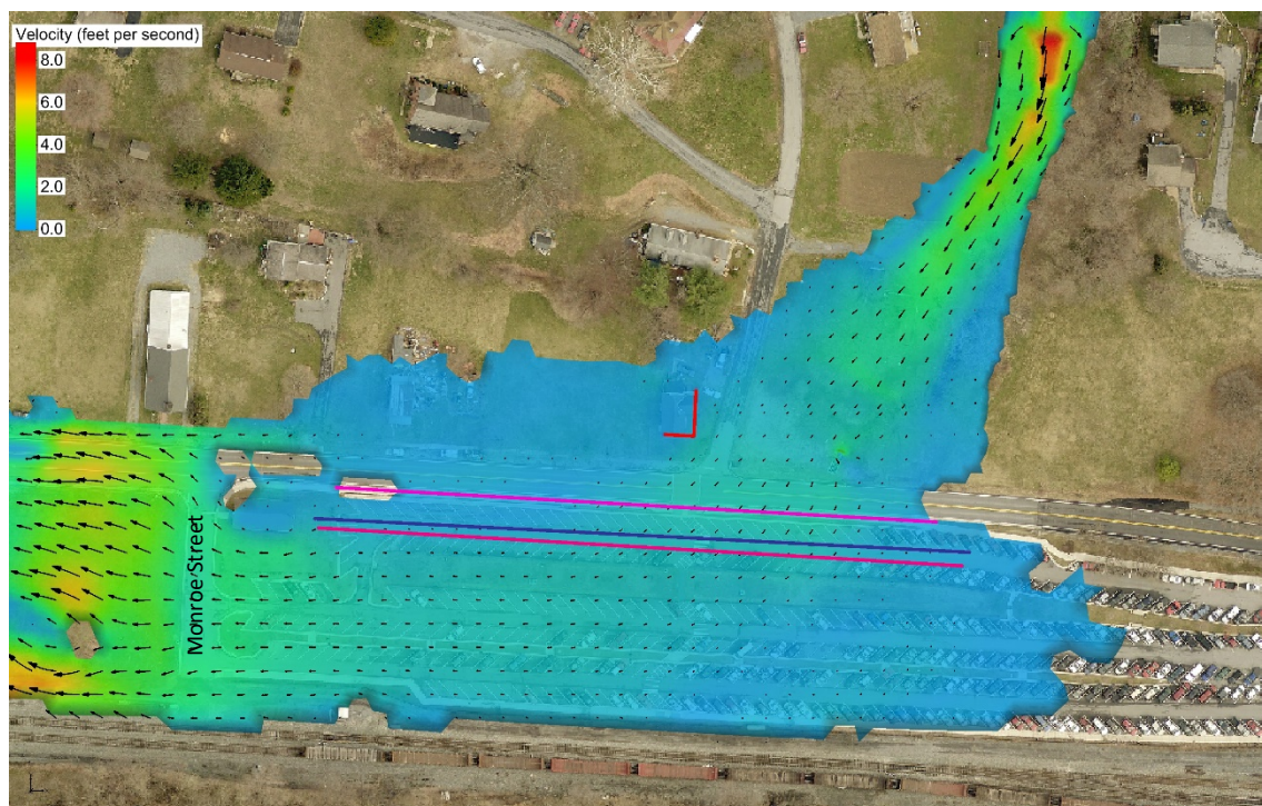
Figure 13. Proposed conditions in the 100-year storm showing the velocity distribution when the maximum depth occurs in the MDOT MTA parking lot. The velocities and depths in the parking lot are controlled by overtopping Monroe Street
