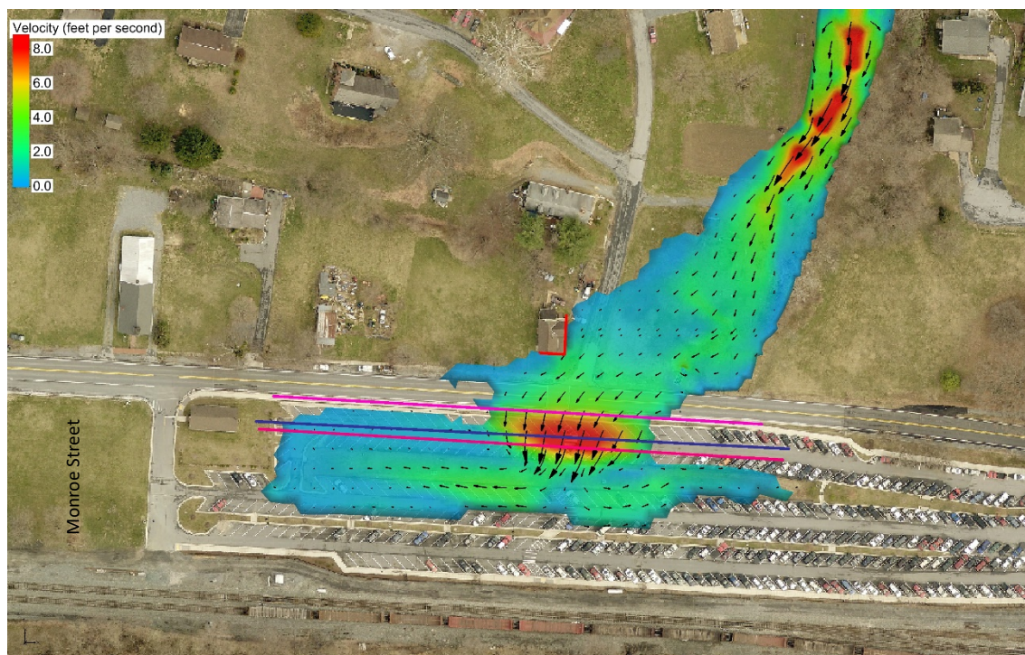
Figure 11. Proposed conditions in the 100-year storm showing the velocity distribution when the maximum velocity occurs in the MDOT MTA parking lot. The red area denoting high velocity is closer to MD-28 in proposed than existing conditions
