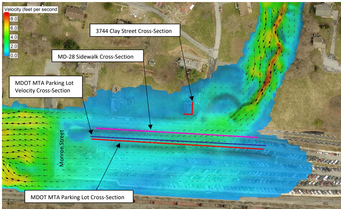
Figure 12. Existing conditions in the 100-year storm showing the velocity distribution when the maximum depth occurs in the MDOT MTA parking lot
