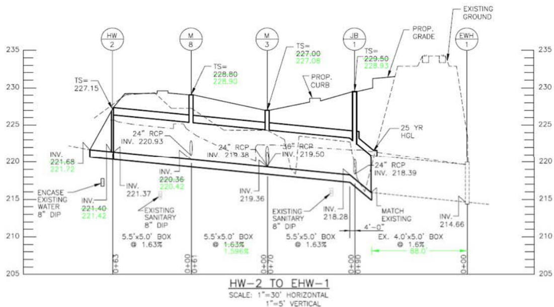
Figure 7. Excerpt from 2008 MDOT MTA Parking Lot As-Built Plans. Note the 5.5 ft x 5 ft culvert joins the legacy 4 ft x 5 ft culvert
