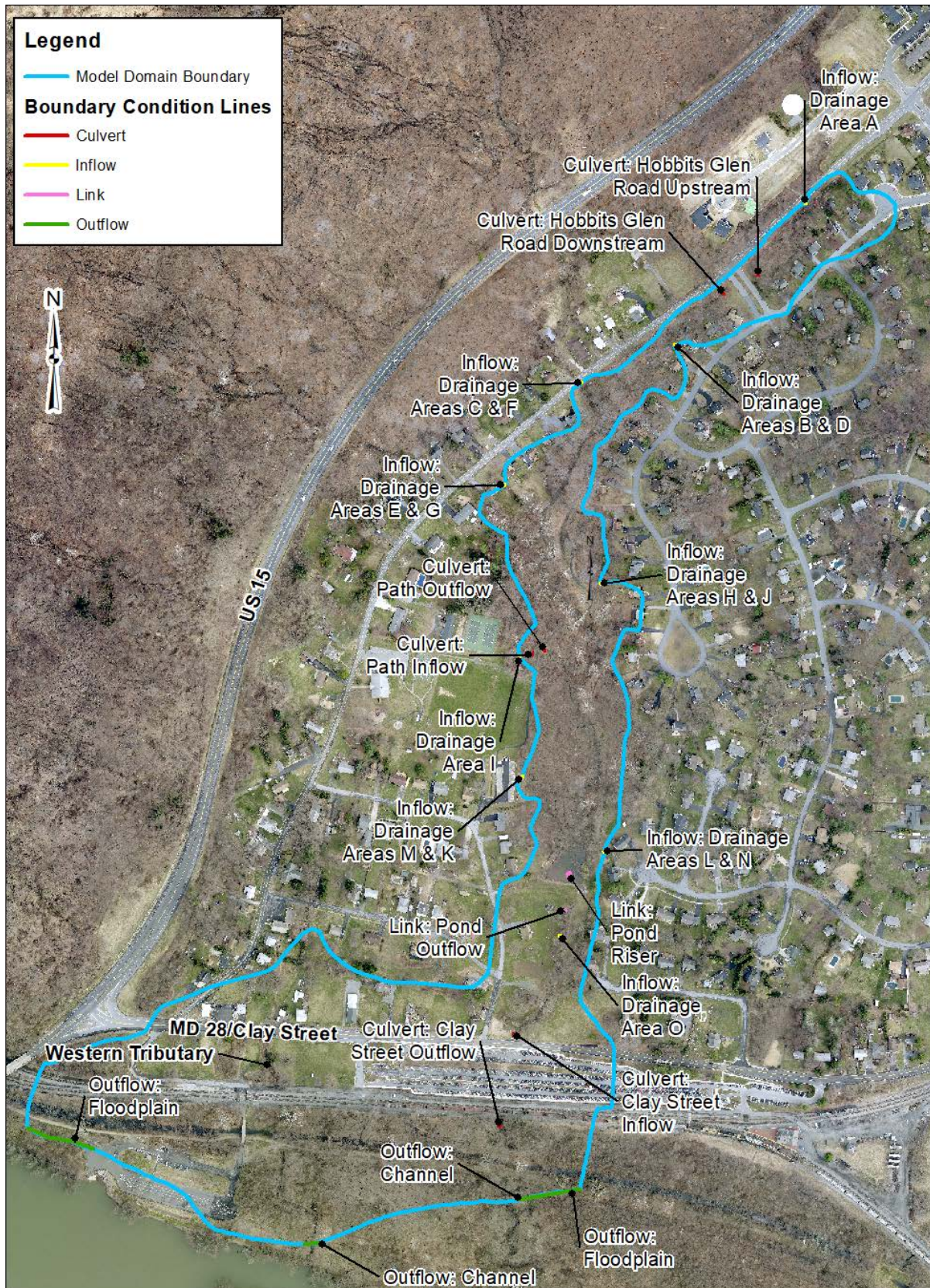
Figure 1. Model Domain and Boundary Condition Locations
