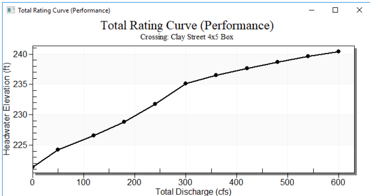
Figure 8. HY-8 Rating curve for MD-28 culvert
