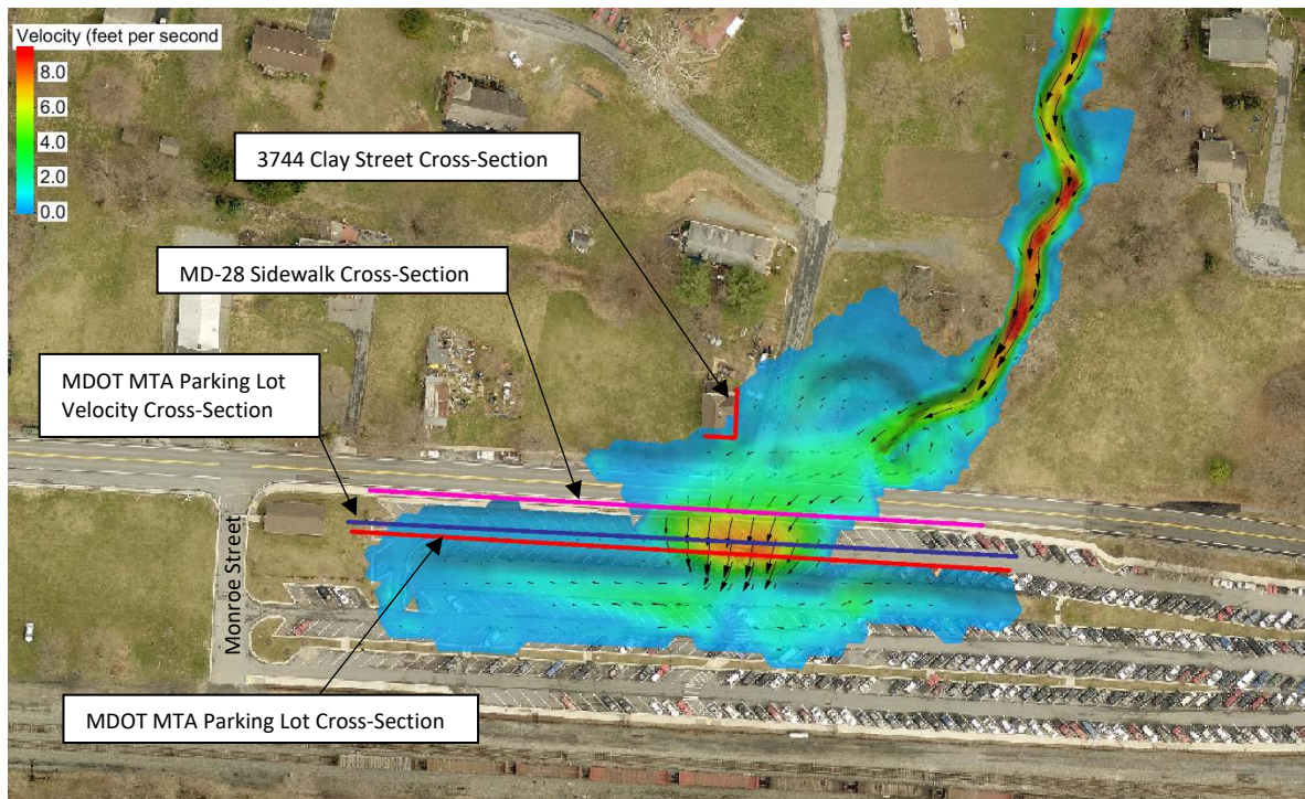
Figure 10. Existing conditions in the 100-year storm showing the velocity distribution when the maximum velocity occurs in the MDOT MTA parking lot
