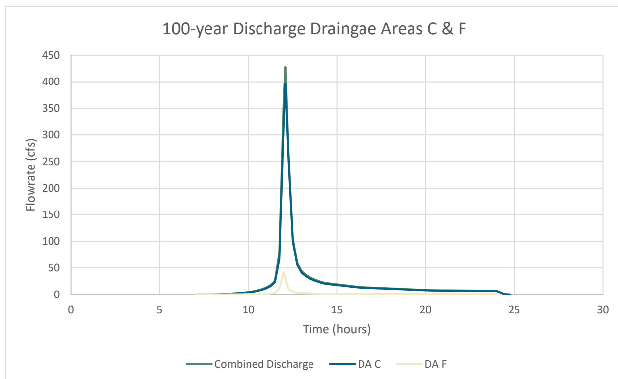
Figure 2. Example Combined Inflow Hydrograph (Drainage areas C & F)
