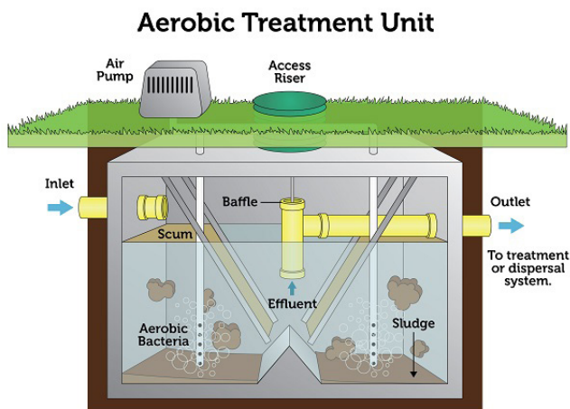
Figure 3: Aerobic Treatment Unit Diagram
